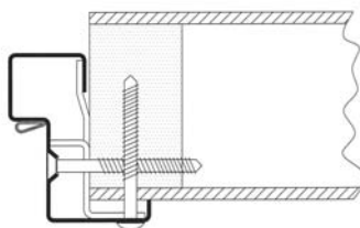
Timber wall
