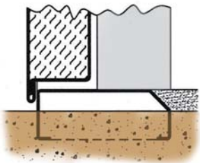
Standard Embedded
