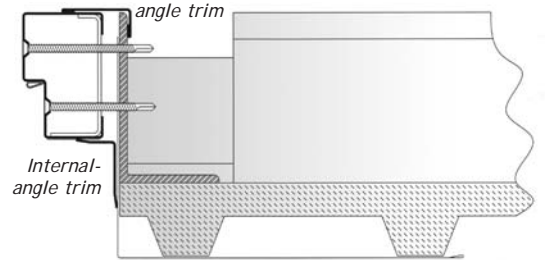
External-angle trim
