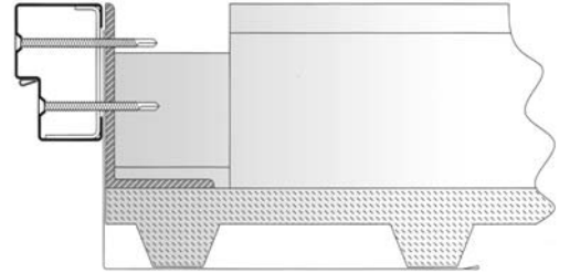
Steel work
