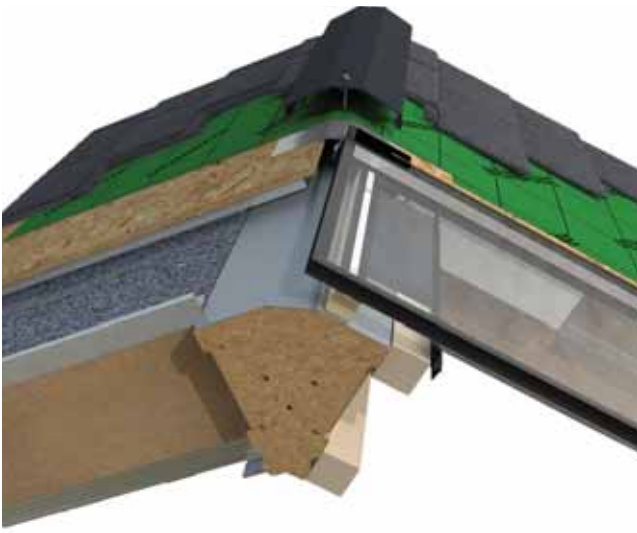
Ridge solid to glass
