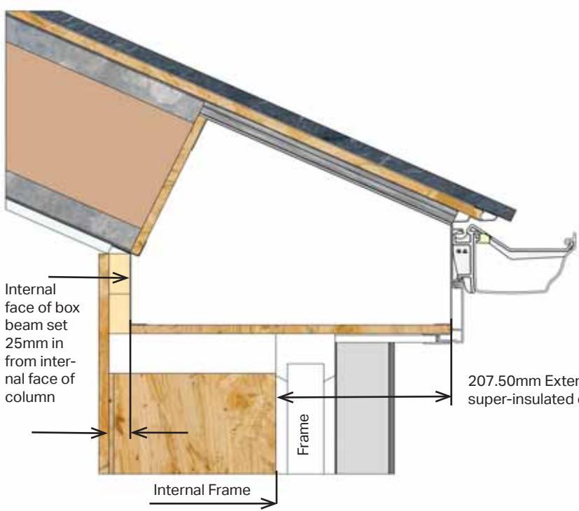
EXTENDED SOFFIT ONLY ON SUPER-INSULATED COLUMN
