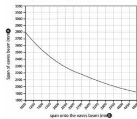
Eaves beam charts based on eaves beam spanning between posts with tie bars aligned with posts / frame stiffener
