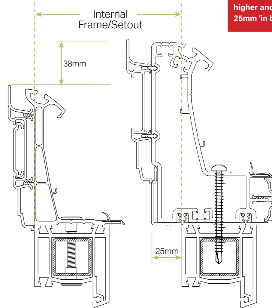
Standard Eaves Beam
