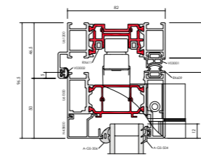
F82 Head
